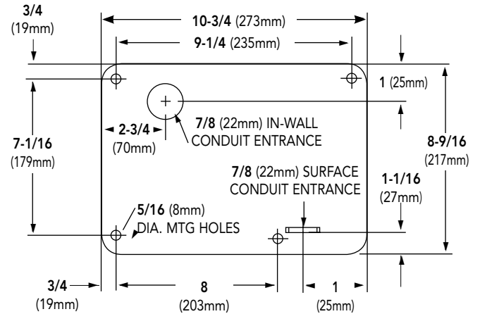
Figure 2 - A-T Series Surface Mount
